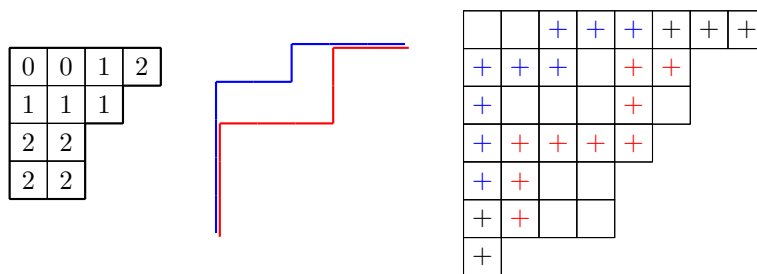
Fig. 6: Reverse plane partition corresponding to Figure 5 and its corresponding 2-fan of paths.
