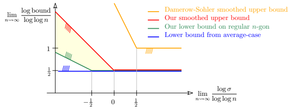
(b) Comparison of the smoothed bounds for Gaussian perturbation in dimension 2 (Theorem 9 and [6]) and the lower bound perturbing the regular n -gon (Theorem 10). A data point with coordinates (x, y) means that for a perturbation of magnitude \sigma = \ln^x n the expected size of the convex hull grows as \ln^y n .
