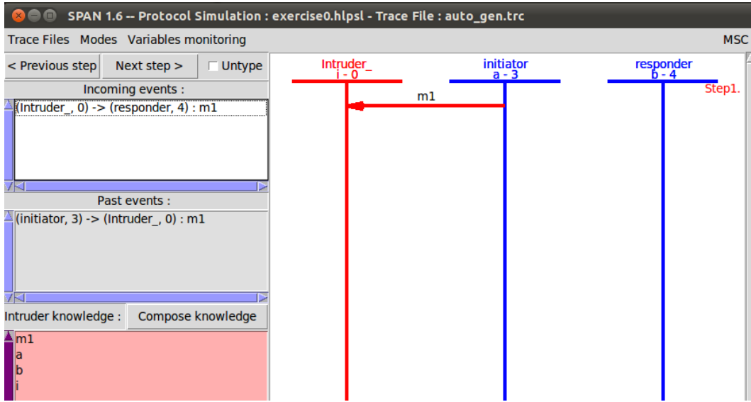
Figure 4: An attack displayed in “Attack simulation” window, with intruder knowledge.
