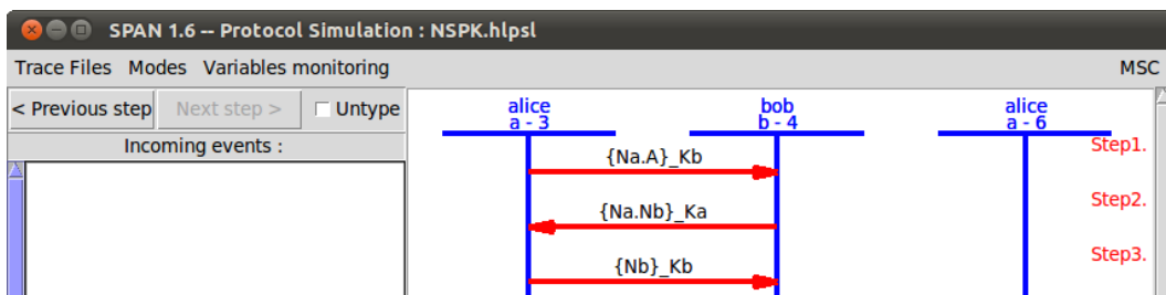
Figure 10: The Needham Schroeder Public Key protocol simulation, with relabelling of arrows.
