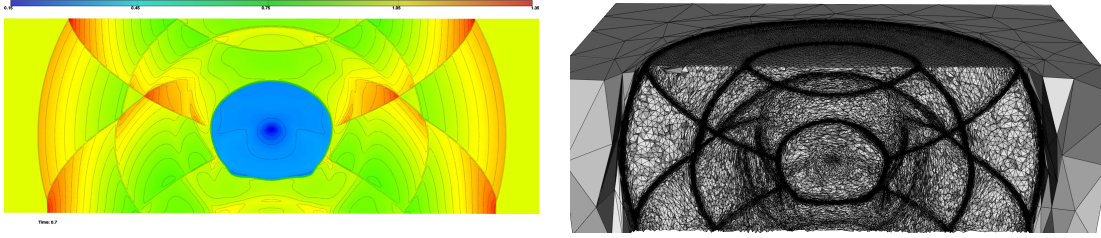
Figure 10: Spherical blast. Reference density solution (left) at a-dimensional time T = 0.7 and final adapted reference mesh (right) containing 2,173,612 vertices and 13,037,975 tetrahedra.
