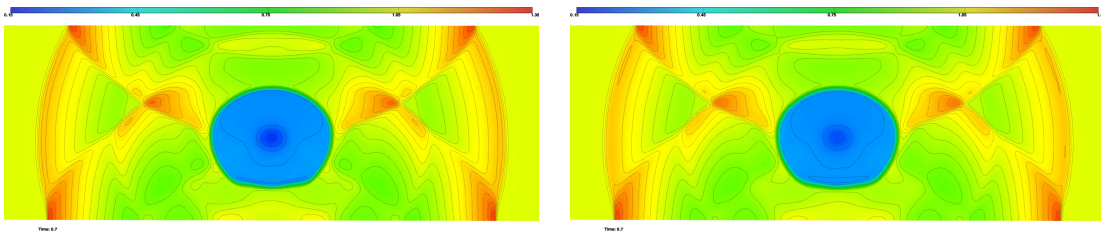
Figure 13: Spherical blast. Density solution at a-dimensional time T = 0.7 obtained with the \mathbb{P}_1 -conservative interpolation (left) and the \mathbb{P}_1 interpolation (right) for n_{\text{adap}} = 16 and \tilde{N}_{\text{ver}} = 240K .
