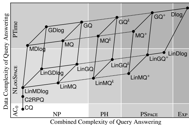
Figure 1: Query languages and complexities; languages higher up in the graph are more expressive
