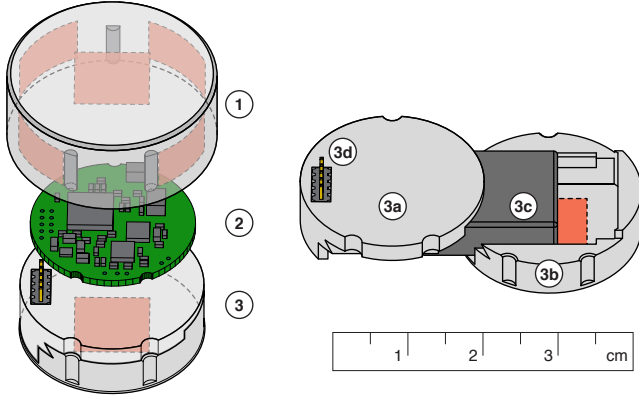
Figure 2. SmartToken Design
