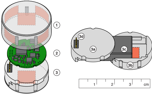
Figure 2. SmartToken Design
