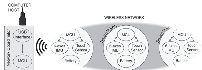
Figure 3. SmartToken Sensor Network Architecture
