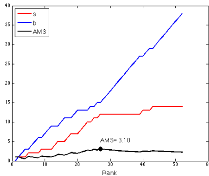
(c) AMS for polynomial
