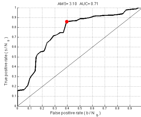
(b) ROC curve for radial
