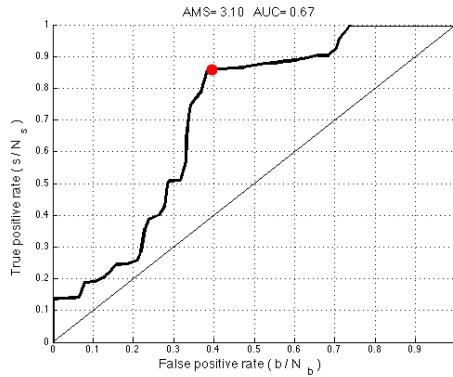
(a) ROC curve for polynomial
