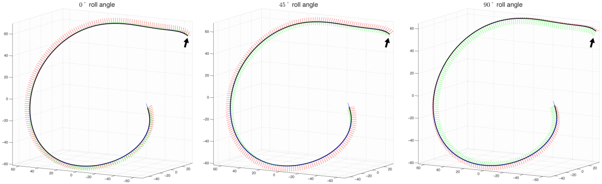
Fig. 4: Different initial roll angles for the parallel transport frame on the same cochlear geometry ( 0^\circ , 45^\circ and 90^\circ ). Red: \mathbf{E}_1 , green: \mathbf{E}_2 .
