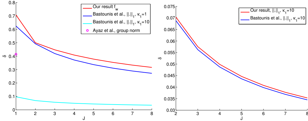
Figure 1: Comparison of our admissible RIP constant and the state of the art (Higher is better). Left : Our result is for weighted group norm with our proposed weights and block group sparsity. Bastounis et al. is for \ell^1 norm and simple sparsity. Ayaz et al. is for the group norm. Right : \kappa_1 = 10 . Our result is for the \ell^1 norm and block sparsity, Bastounis et al. is for the \ell^1 norm and block sparsity.
