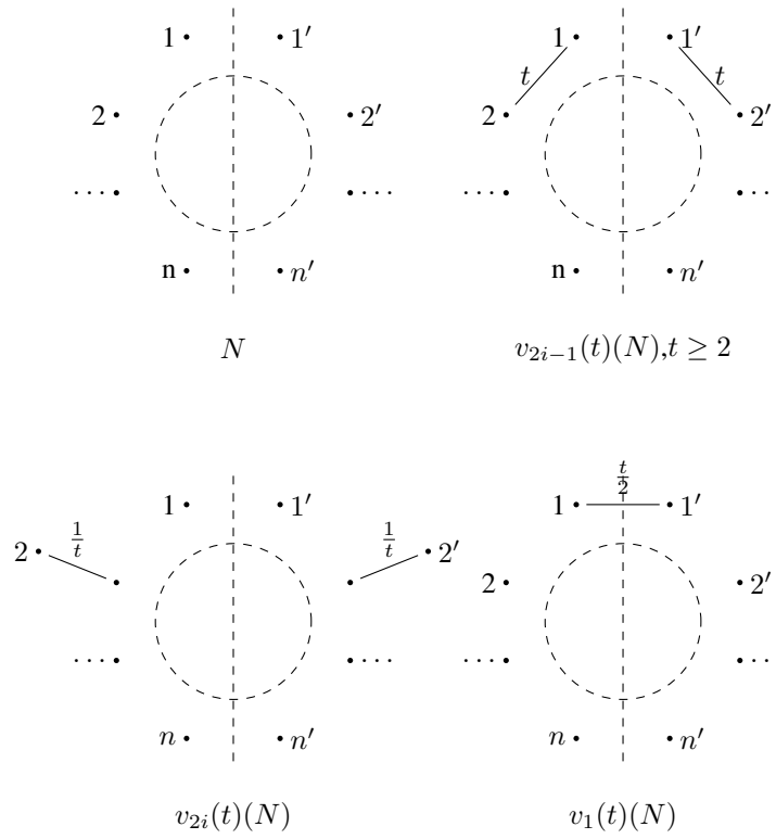
Fig. 6: (E_{B_{2n}})_{\geq 0} action
