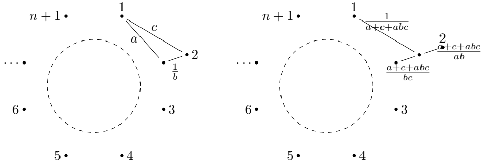
Fig. 3: Braid relation
