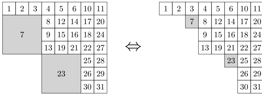
Fig. 11: The correspondence between ((k^n), (r), (s)) -Young books and standard Young tableaux of truncated shape in Figure 10.
