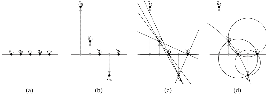
Fig. 1: A point configuration \{a_1, \dots, a_5\} (a) and one of its D -liftings \{\hat{a}_1, \dots, \hat{a}_5\} (b). It fulfills conditions (i) (c) and (ii) (d). It is not a positive D -lifting since the height of \hat{a}_4 is negative.
