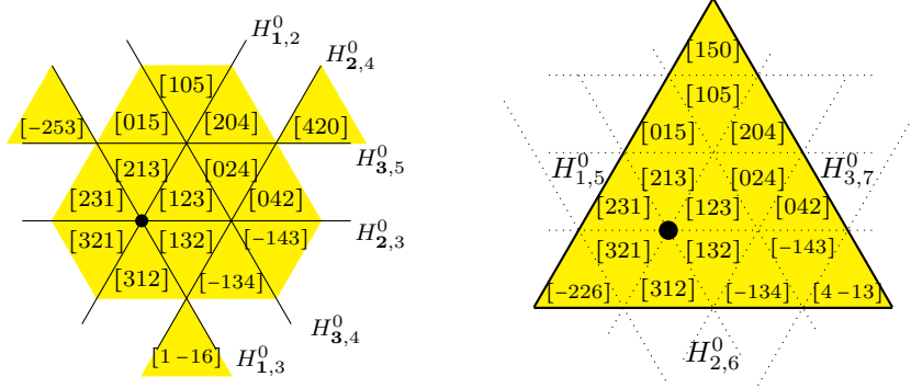
Fig. 4: m = 4, n = 3 On the left, minimal alcoves \omega(A_0) for \text{Sh}_3^1 are labeled by \omega \in \tilde{\mathcal{S}}_n^m . On the right, alcoves \omega^{-1}(A_0) fit inside D_3^4 , labeled \omega^{-1} \in {}^m \tilde{\mathcal{S}}_n .
