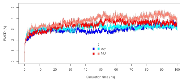
Figure 3: RMSD for the Growth Hormone Complex. Colors correspond to the two replicates (1 and 2) of the WT and MU.
