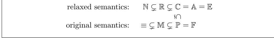
Figure 8: Relationships between the equivalences of \lambda_S
