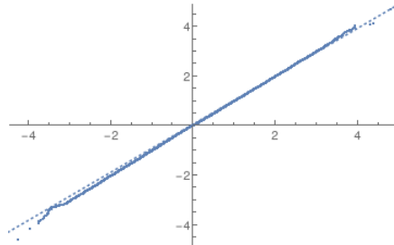
FIG 2. A Q-Q plot between the first algorithm and the SBM's exact algorithm for a skew Brownian motion with \beta = 0.7 starting from 0.
