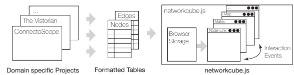
Figure 3: NetworkCube pipeline
