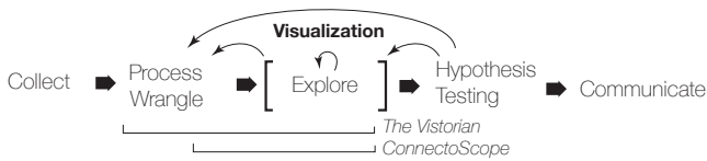
Figure 2: Exploration workflow
