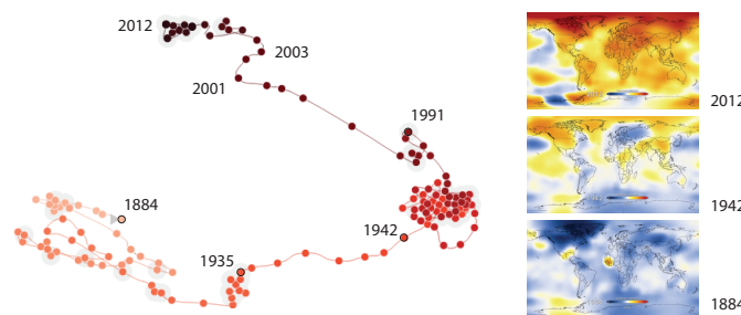
Fig. 10. Evolution of global temperature between 1884 and 2012. The backtracking is an artefact of video analysis (see stills on the right).
