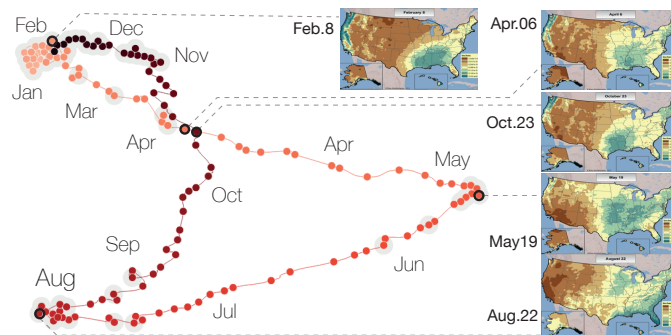
Fig. 9. Precipitation in the US across one year.
