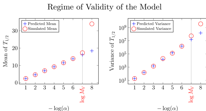
FIG. 4. Comparison between the simulations and the predictions to see the regime of parameters where the calculations are valid. For these simulations, we fixed M_V = 10^7 monomers, \beta = 1 , and made \alpha varying.
