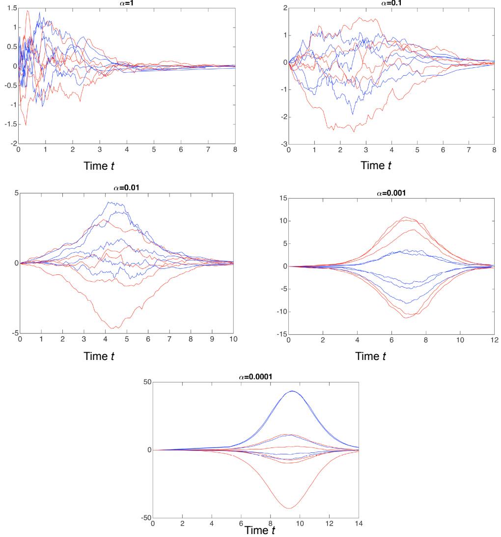
FIG. 8. For each of the previous values of \alpha = 10^{-k} with k = 0, \dots, 4 five trajectories for U_V in blue and five trajectories for U in red, for M = 10^5 . We see that the noise inside each path decreases when \alpha decreases, the stochasticity remaining in the startup of the curves.
