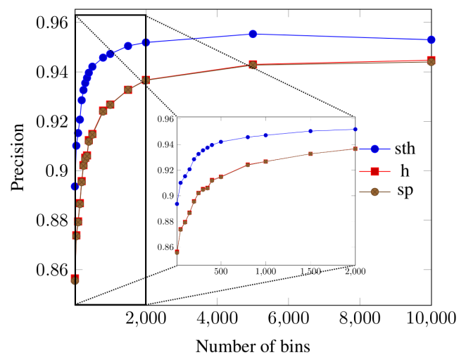
Figure 4: Evolution of the precision as the number of bins in the descriptors increases, from 10 to 10,000 bins. The curves of color histograms and spatiograms are overlapping.
