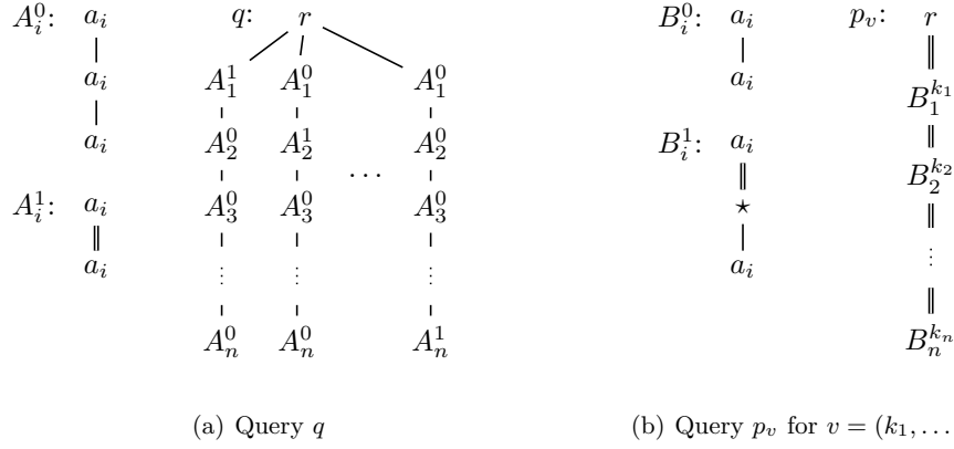
■ Figure 2 Twig query q requiring exponentially many examples w.r.t. p_v .
