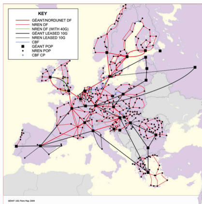
Figure 1: The European GÉANT backbone
