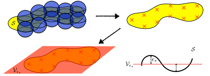
Figure 1. Construction of \mathcal{V}_{\epsilon_*} . Top left: cover of \mathcal{S} with N(\epsilon_*) balls of radius \epsilon_* . Top right: the centres of the balls, indicated by the red crosses, form a \epsilon_* -net, denoted by \mathcal{C}(\epsilon_*) , for \mathcal{S} . Bottom left: the linear span of the vectors in \mathcal{C}(\epsilon_*) is \mathcal{V}_{\epsilon_*} . Bottom right: \mathcal{V}_{\epsilon_*} approximates \mathcal{S} with precision \epsilon_* .
