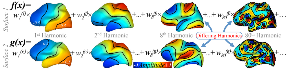
Fig. 1. Spectral Decomposition on Shapes – Any function f(x) on surface 1 ( top row ), or g(x) on surface 2 ( bottom row ) can be written as a sum of weighted harmonics (coloring is harmonic amplitude). Spectral weights, \mathbf{w}^{(f)} and \mathbf{w}^{(g)} , are not directly transferable between surfaces since harmonics may change sign (bases 8), and not correspond (differences in black isolines, incompatible bases 80).
