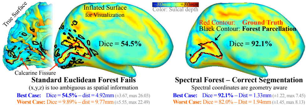
Fig. 2. Segmentation of the Calcarine Fissure – which is deeply buried in a highly convoluted area. (Left) Learning surface data with forests on standard Euclidean features produces low Dice scores, and a segmentation that is spatially inconsistent. (Right) Spectral Forests directly learn surface data via spatial features that are geometry aware. Surfaces are inflated only for visualization.
