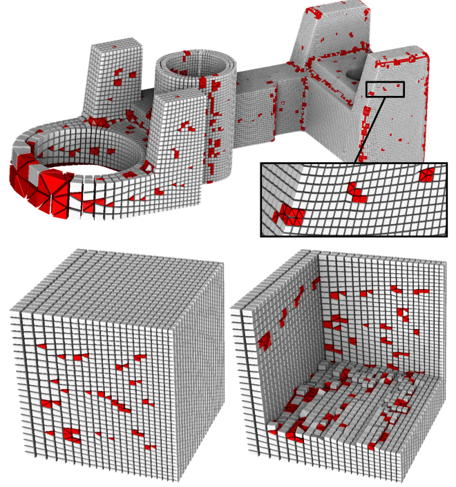
Fig. 14: Varying scale: In the upper image, the desired hexahedra size varies linearly with the x coordinate. The bottom row shows a cube (clipped on the right image) with a varying anisotropic scale. Singularities are evenly distributed to absorb the variation of resolution.
