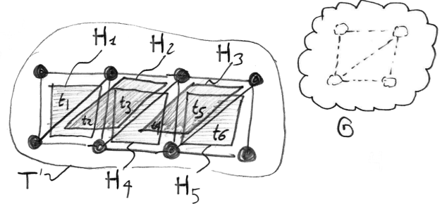
Fig. 8: Recombination (in 2D): the template G describes the recombination of two triangles into a quad. Five instances H^* = \{H_1, H_2, H_3, H_4, H_5\} can be found in the intermediate mesh T' . Clearly, H_2 and H_3 are of lower quality (lower value of function Q ). H_1 and H_2 are mutually incompatible ( C(H_1, H_2) = 1 ) because they have t_2 in common. The other mutually incompatible pairs are (H_2, H_4) , (H_4, H_3) and (H_3, H_5) .
