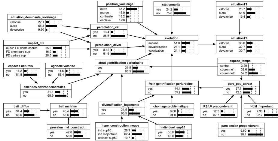
Fig. 1. The BN model for the valorization/devalorization of municipalities in the study area (from [15]).
