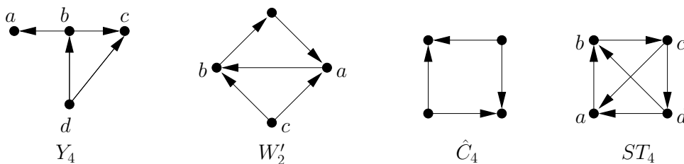
Figure 7: The oriented graphs Y_4 , W'_2 , \hat{C}_4 , and ST_4
