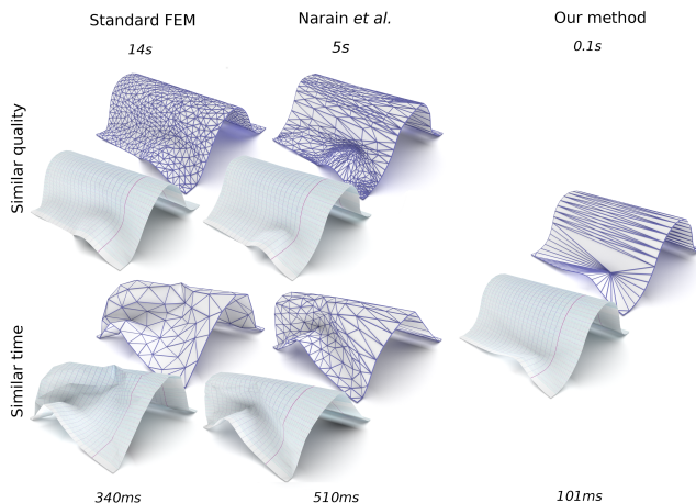
Fig. 19. Comparison with other methods. The upper row shows how much mesh refinement is required for Standard FEM (top left) and Narain et al. [2013] method (top middle), in order to get a result of similar visual quality as our method (right).
