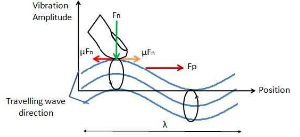
Fig. 4. Principle of the friction reduction by travelling wave
