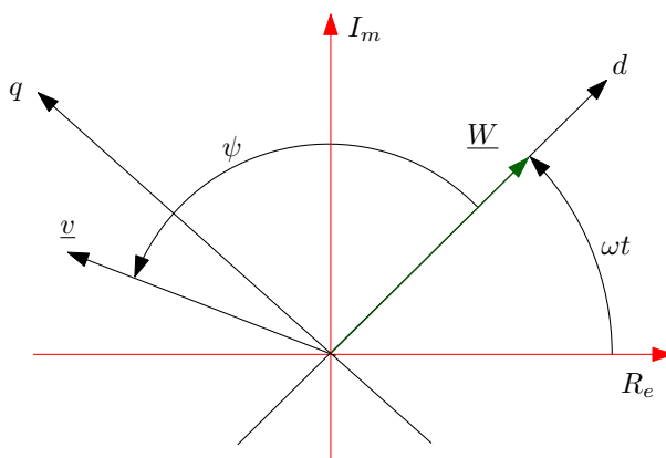
Figure 3: Representation of the vibration amplitude and the voltage in a rotating reference frame
