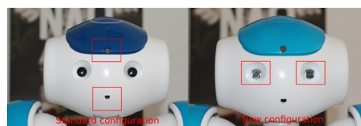
Figure 3: The standard NAO head (left) includes two vertically aligned cameras with no common field of view (top camera is heading upwards while bottom camera is heading downwards). Recently, Aldebaran Robotics developed a prototype stereo head (right). The wide field of view shared by the cameras enables stereo matching and stereo reconstruction.
