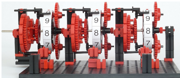
Figure 23: Püttmann's simplified reconstruction of Chebyshev's adding machine. ( https://fischertechnikblog.wordpress.com )
