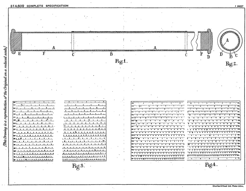
Figure 18: Figure from Podtiaguin's British patent [48] (1928).
