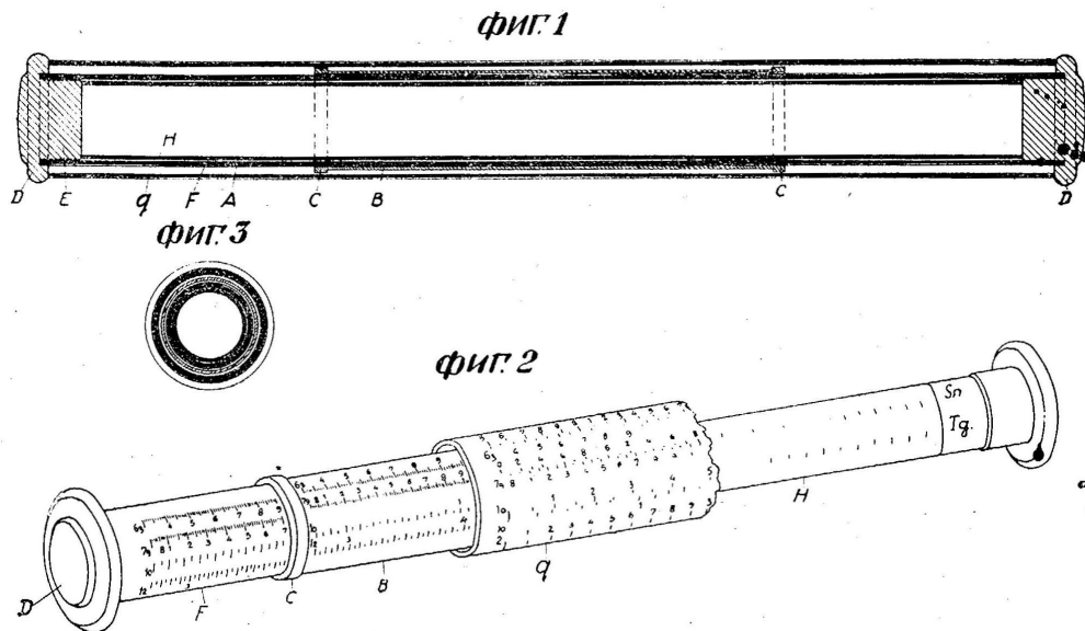
Figure 16: Figure from Podtiagin's soviet patent [49] (1926).
