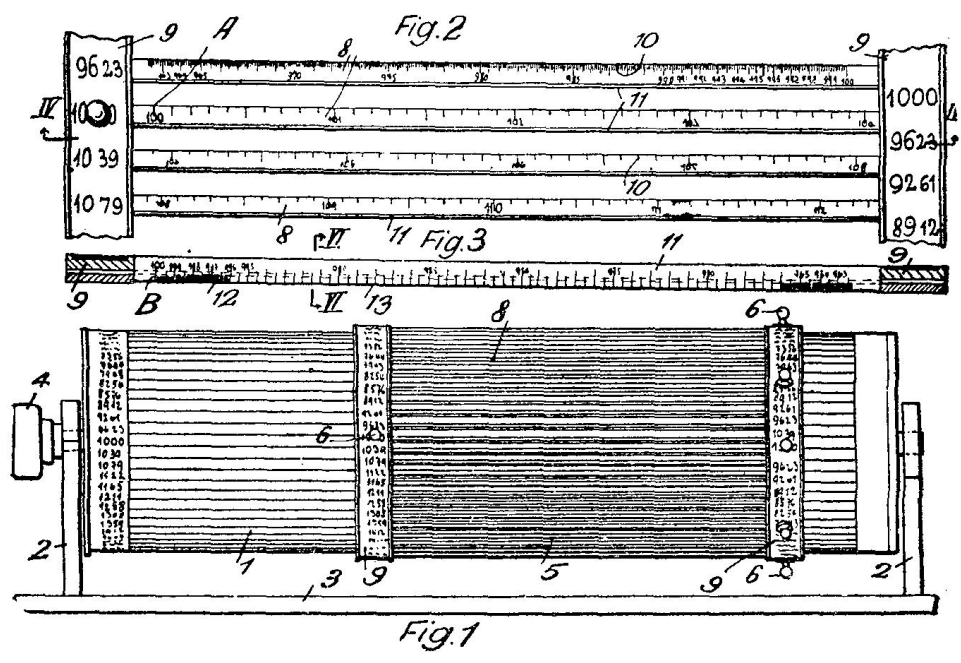
Figure 11: Figure from (Max) Billeter and Bohnhorst's patent on a calculating cylinder [8] (1917).
