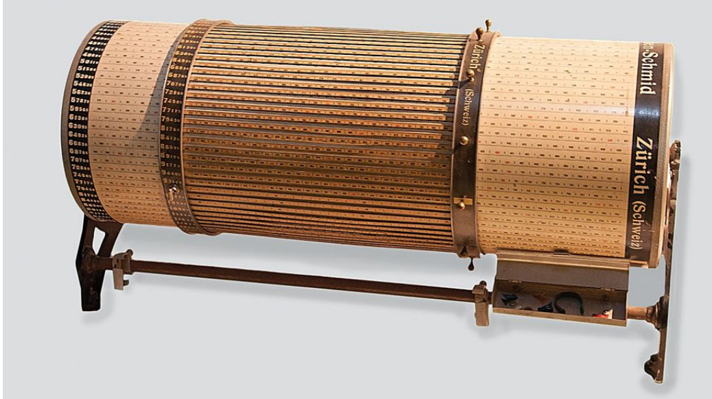
Figure 14: A 24 m LOGA cylindrical slide rule at UBS Basel. (picture provided by Céline Rader, UBS, reproduced with permission)
