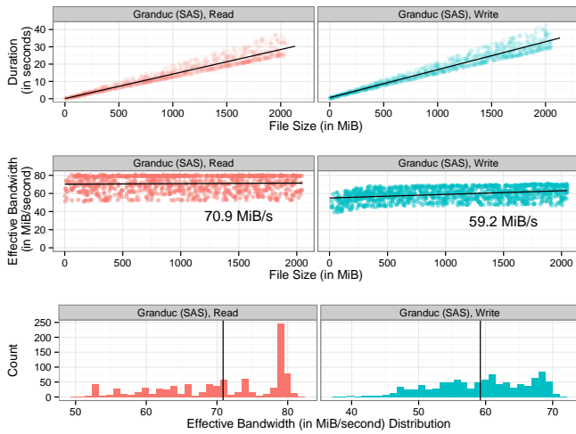
Figure 6. Characterization of read (left) and write (right) operation vs. file size on the SAS disks of the Granduc cluster.
