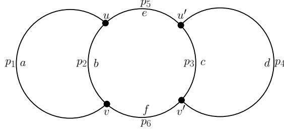
Fig. 1: A generalized polygon tree with three interior regions.
