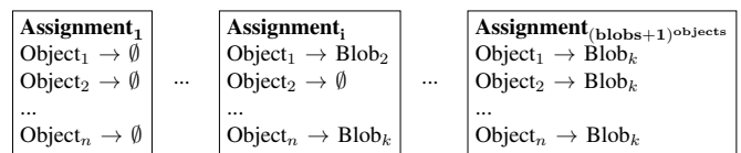
Figure 9: All the possible assignments of known objects to blobs are evaluated and ordered according to how well the blobs are matched in terms of weight by their contents. The assignment having the minimal weight mismatch is considered as most probable.
