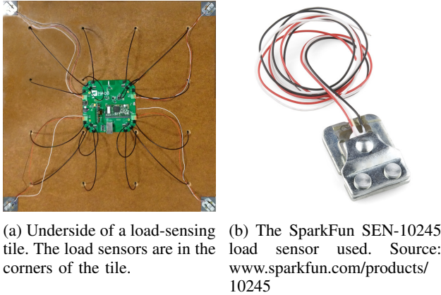
Figure 1: An image of a tile and a load-sensor.
