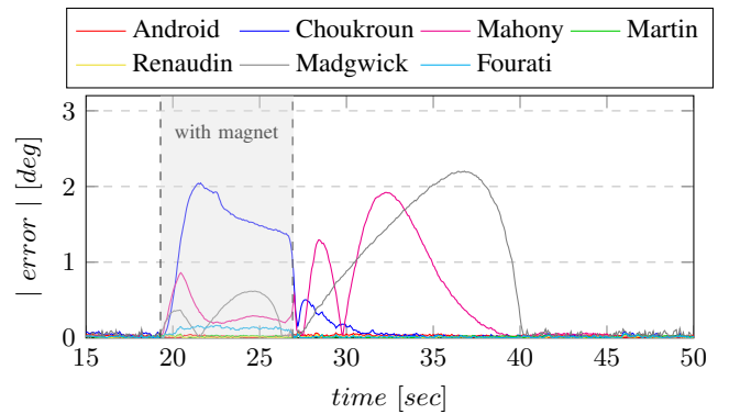
Fig. 13. Precision error on pitch component with a magnet distortion.
