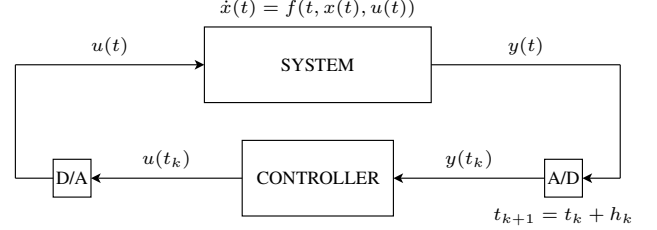
Fig. 1: Sampled-data system
