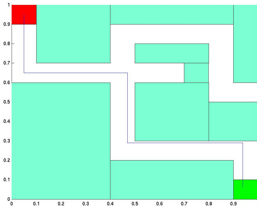
Figure 1: The Maze and the mouse trajectory according to BOCOPHJB
