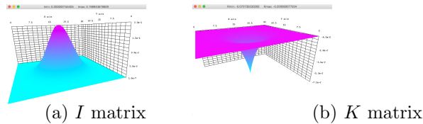
Figure 3. Breather parameters plotted in the simulator for I and K in Eq. (1).
