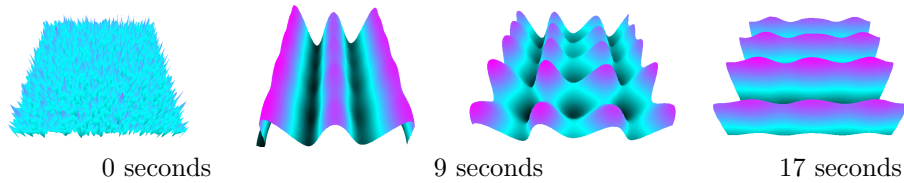
Figure 6. Turing patterns in neural field activity forming over time during the same simulation.
