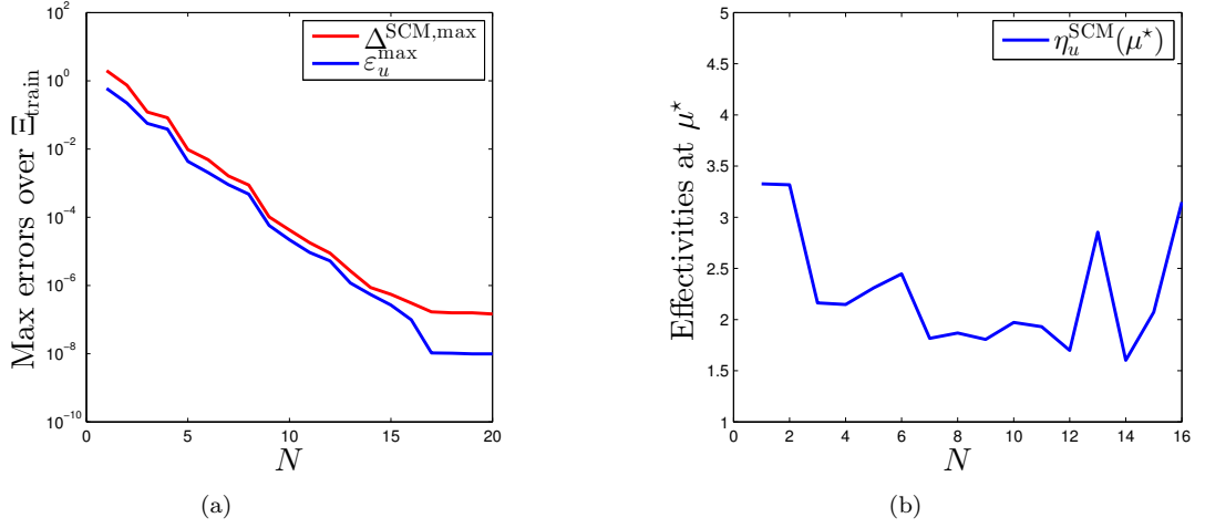
Figure 7: (a) Maximum of SCM upper error bound \Delta^{\text{SCM,max}} and displacement RB error \varepsilon_u^{\text{max}} over E_{\text{train}} , and (b) displacement effectiveness at \mu^* as functions of N (only first 16 iterations are shown in fig. 7(b)).
