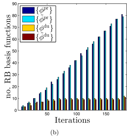
Figure 17: (a) Maximum of \text{gap}_{G,\lambda} , \text{gap}_G and \text{gap}_\lambda over \Xi_{\text{train}} , and (b) sizes of the sets \mathcal{Z}^{\text{pr}} , \tilde{\mathcal{Z}}^{\text{pr}} , \mathcal{Z}^{\text{du}} and \tilde{\mathcal{Z}}^{\text{du}} as functions of GO-greedy iterations.
