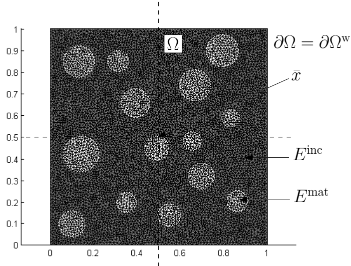
Figure 3: The finite element discretisation of the parametrised SVE.
