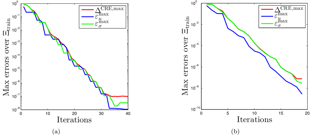
Figure 9: Maximum of relative errors using: (a) our proposed TF-greedy algorithm and (b) TF-greedy algorithm enriching both fields simultaneously at one iteration.
