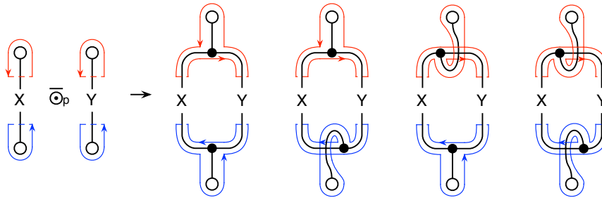
Fig. 5: Production: uu_i^\bullet \overline{\odot}_p uu_j^\bullet \longrightarrow 4uu_{i+j+1}^\bullet .
