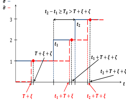
Fig. 4. Dwell time. Note that when a change between sets \Omega_s^\delta is detected the discrete state estimation is maintained in the past value.
