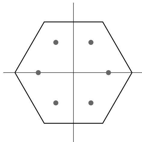
(b) Orbits with m=6 nodes: 2 on the x_1 -axis
