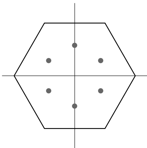
(c) Orbits with m=6 nodes: 2 on the x_2 -axis
