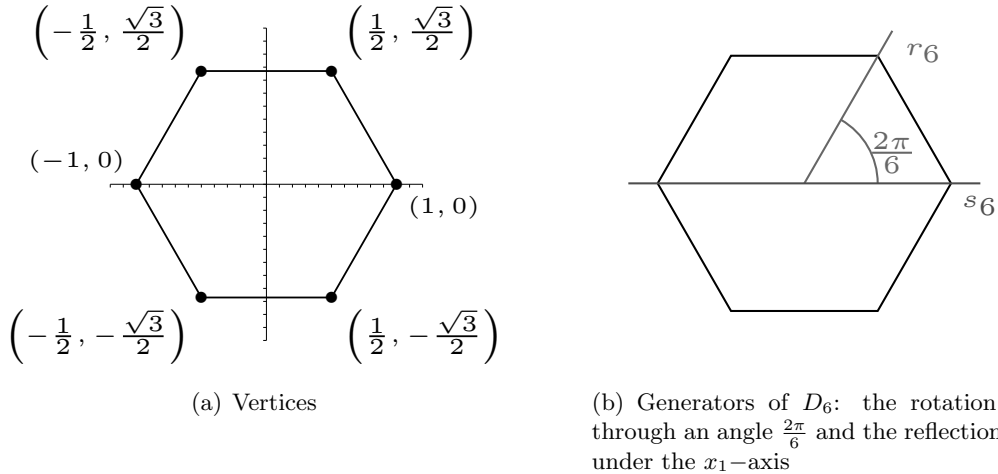
Figure 5: Regular hexagon H_2
