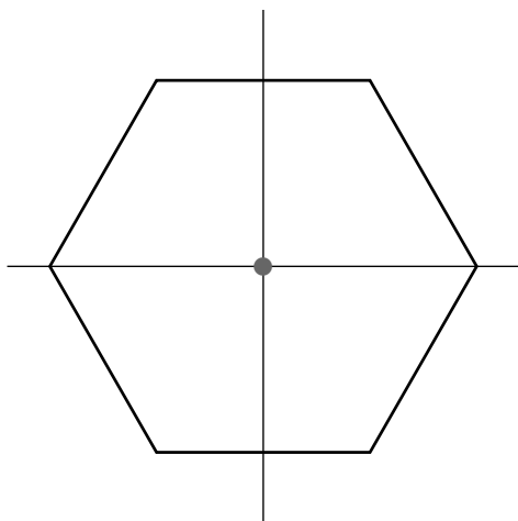
(a) The origin
