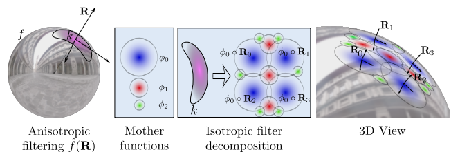
Fig. 1. Illustrating the ISD: we decompose an input filter (in purple) into a sum of displaced copies of a single isotropic mother kernel \phi_i at each frequency band l . This allows us to efficiently filter the input signal with any rotated version of the anisotropic kernel, all with only a few lookups into prefiltered data.
